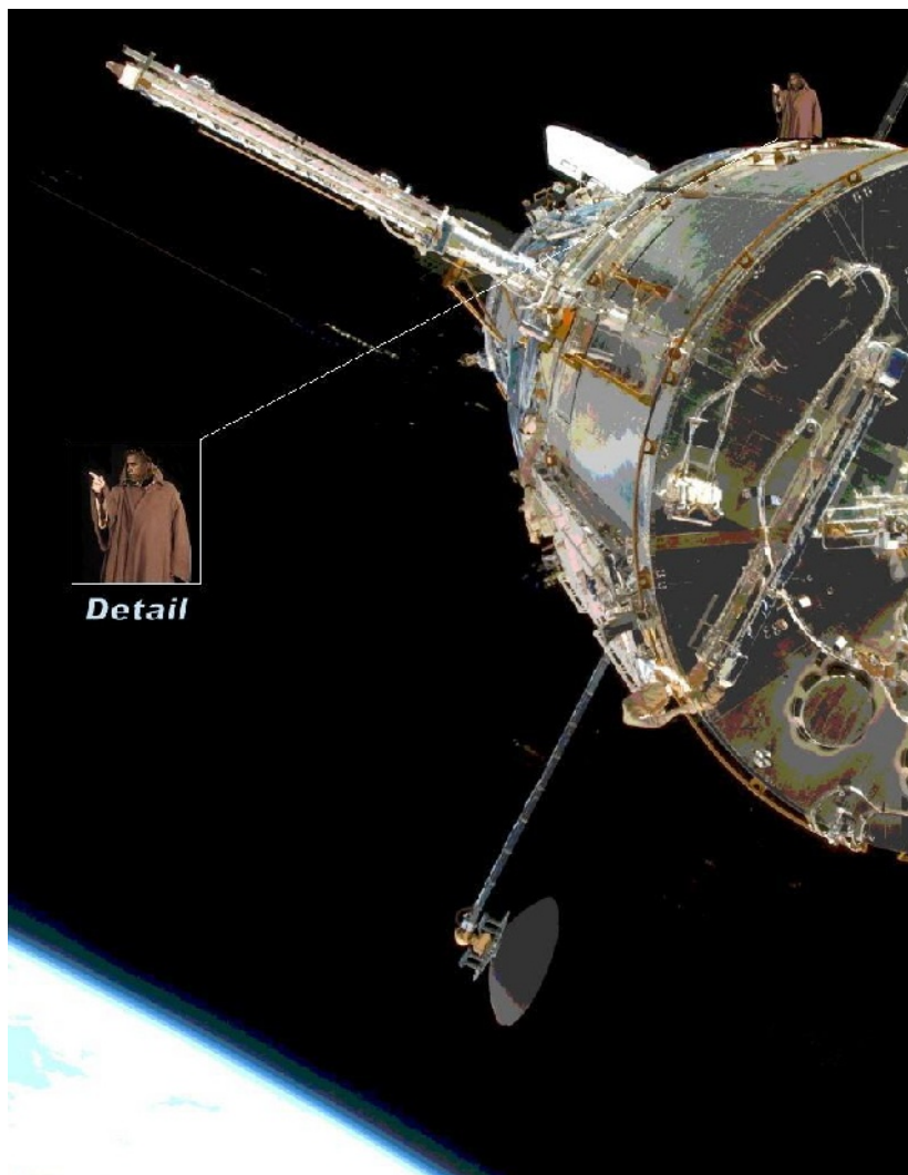
Hubble Photo from NASA, Detail picture from anon.
